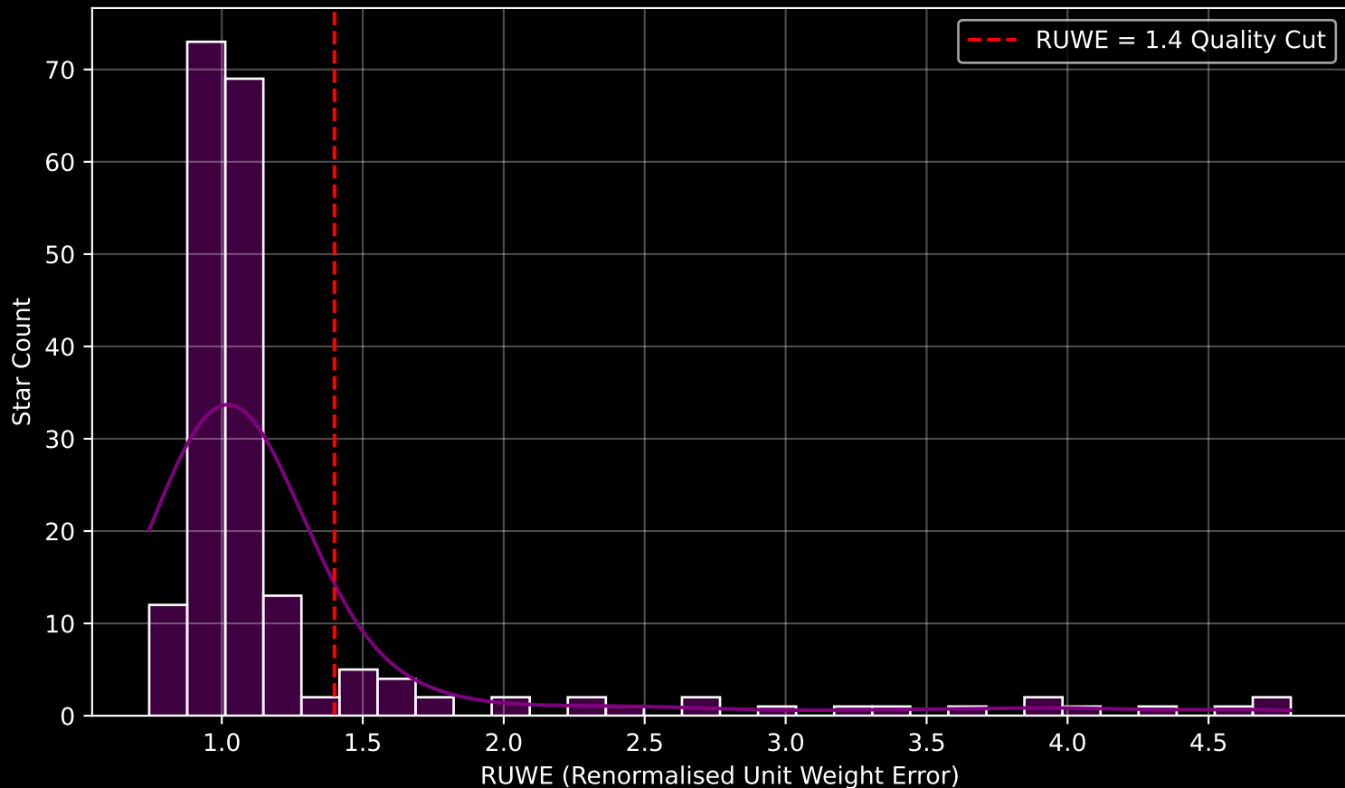
GAPOGEE DR17 Field [088+55_MGA] RUWE Distribution (n= 198)
