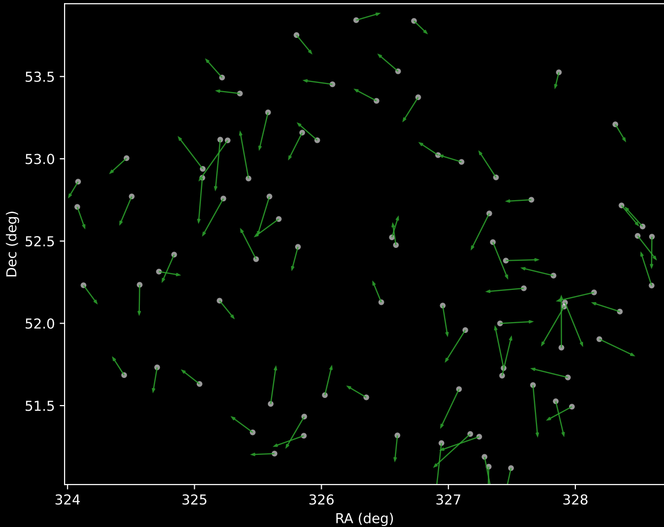
APOGEE DR17 Cluster 4 Proper Motion Vectors (n=83)
