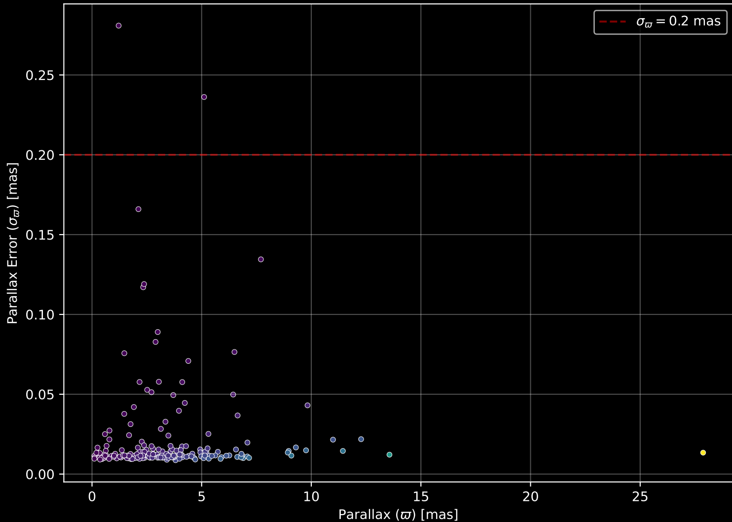
APOGEE DR17 Field: [088+55_MGA] Parallax Quality (n= 211)
