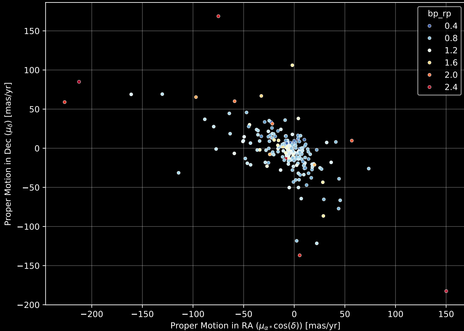
APOGEE DR17 Field: [088+55_MGA] Proper Motion Diagram (n= 211)
