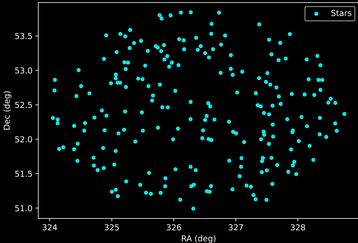
APOGEE DR17 Field: [088+55_MGA] Proper Motion Vectors for Gaia Star Field (n= 211)
