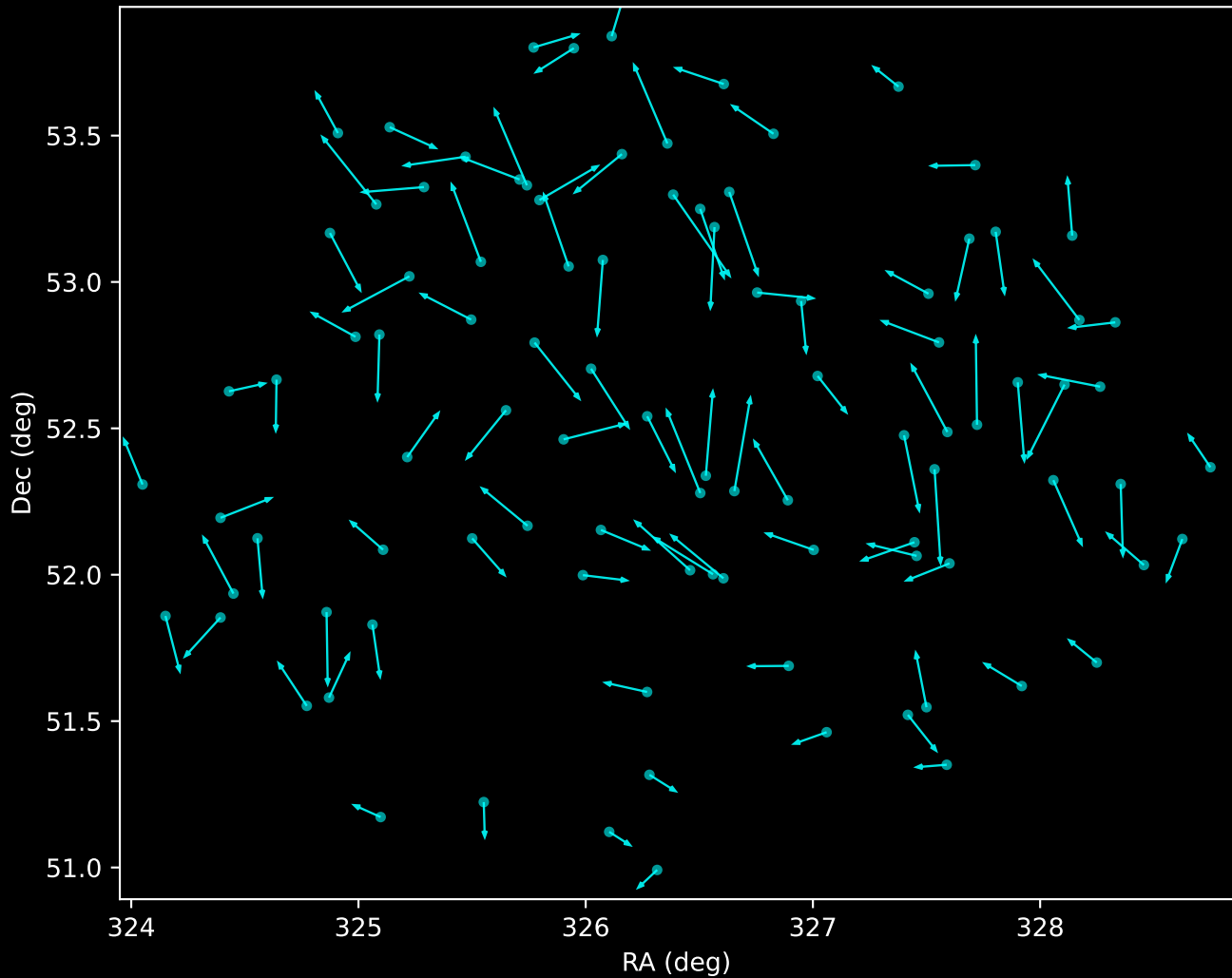
APOGEE DR17 Noise Stream Proper Motion Vectors (n=98)
