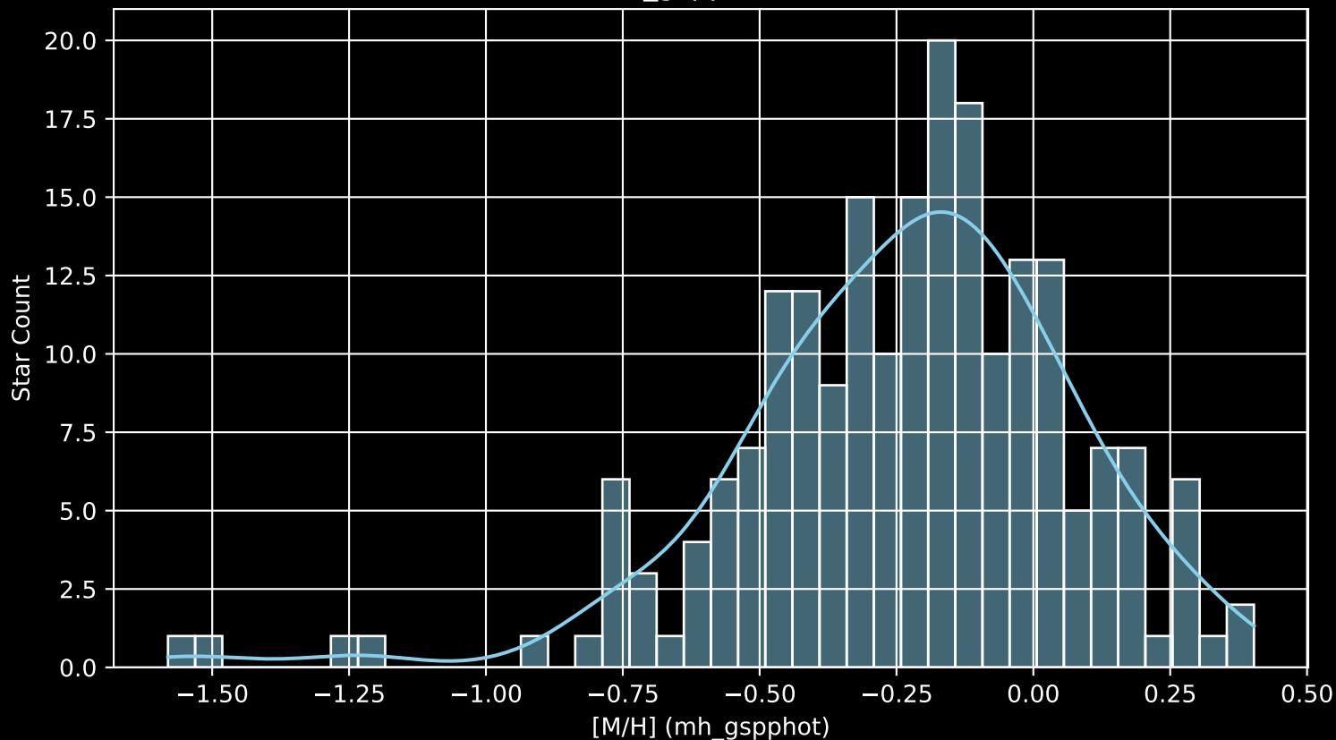
APOGEE DR17 Field: [088+55_MGA [M/H] (mh_gspphot) (n= 209)
