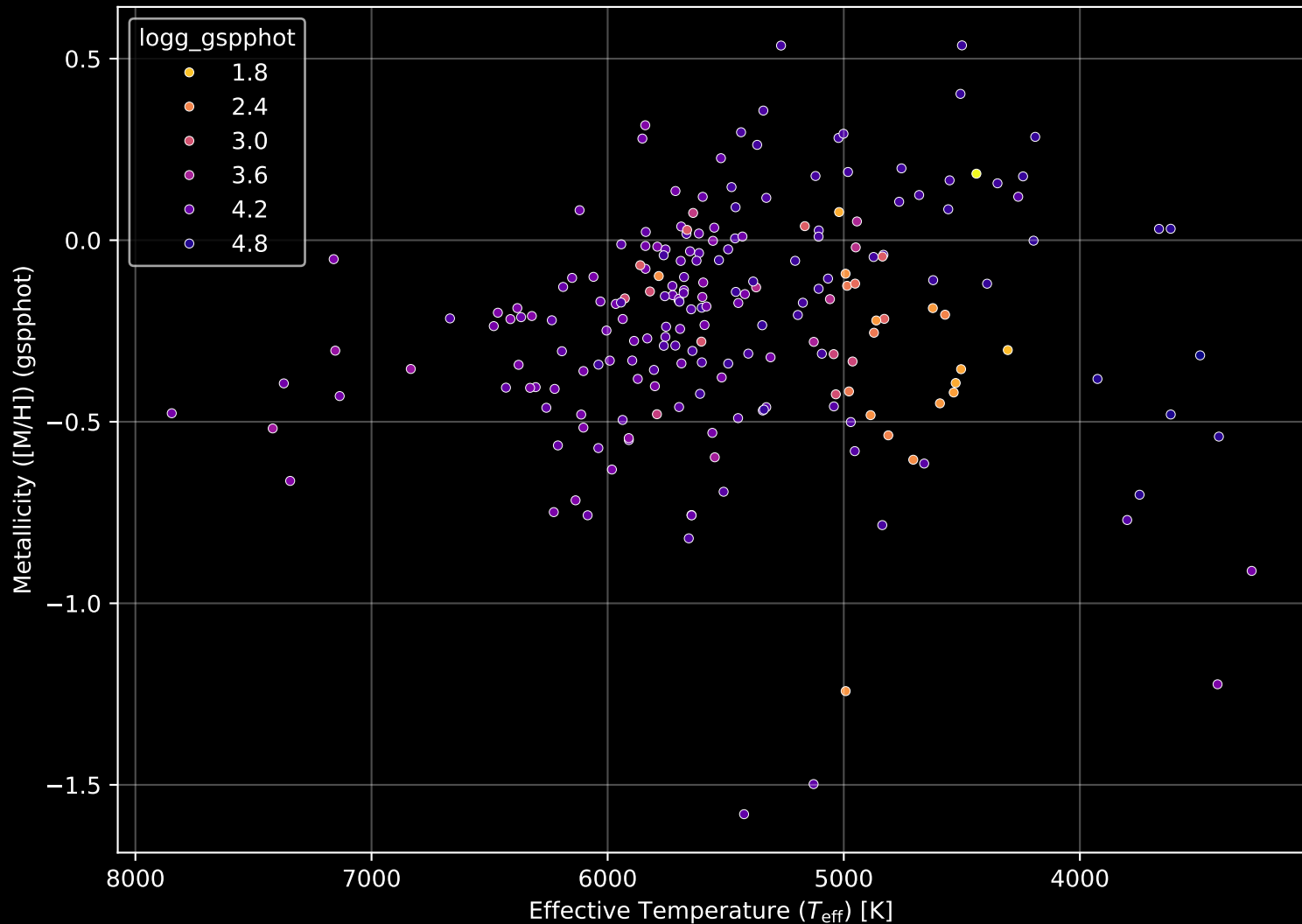
APOGEE DR17 Field: [088+55_MGA] Stellar Population Parameters (n= 211)
